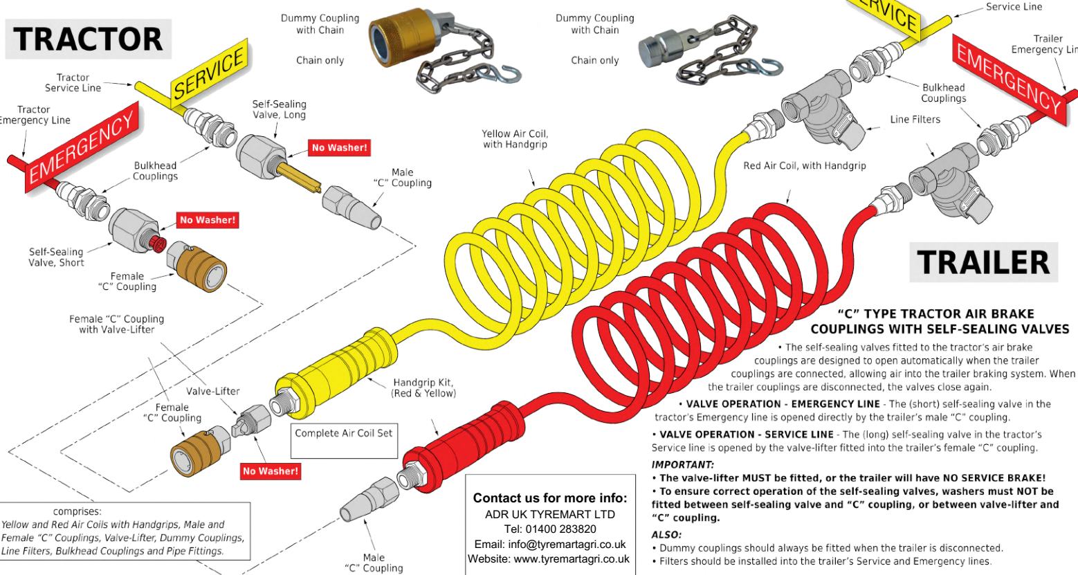
Male "C" Coupling with Self-Sealing Valve, Long
